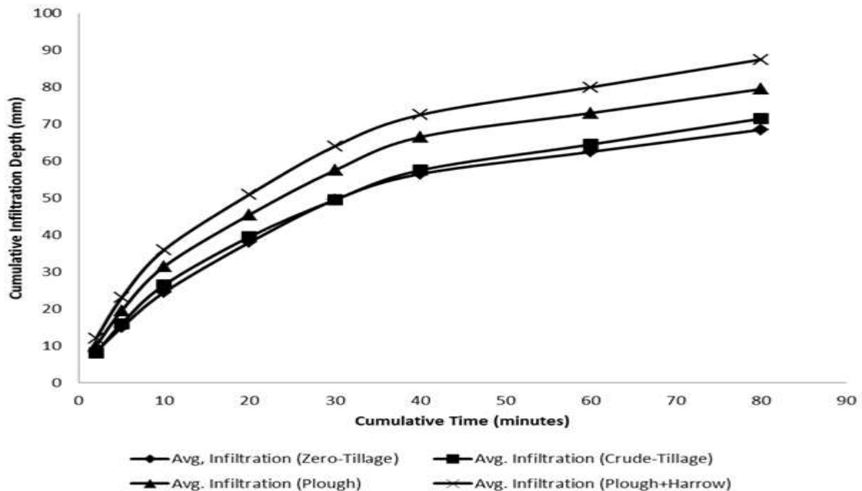
Figure-4. Comparative Infiltration Curves for Different Tillage Treatments
