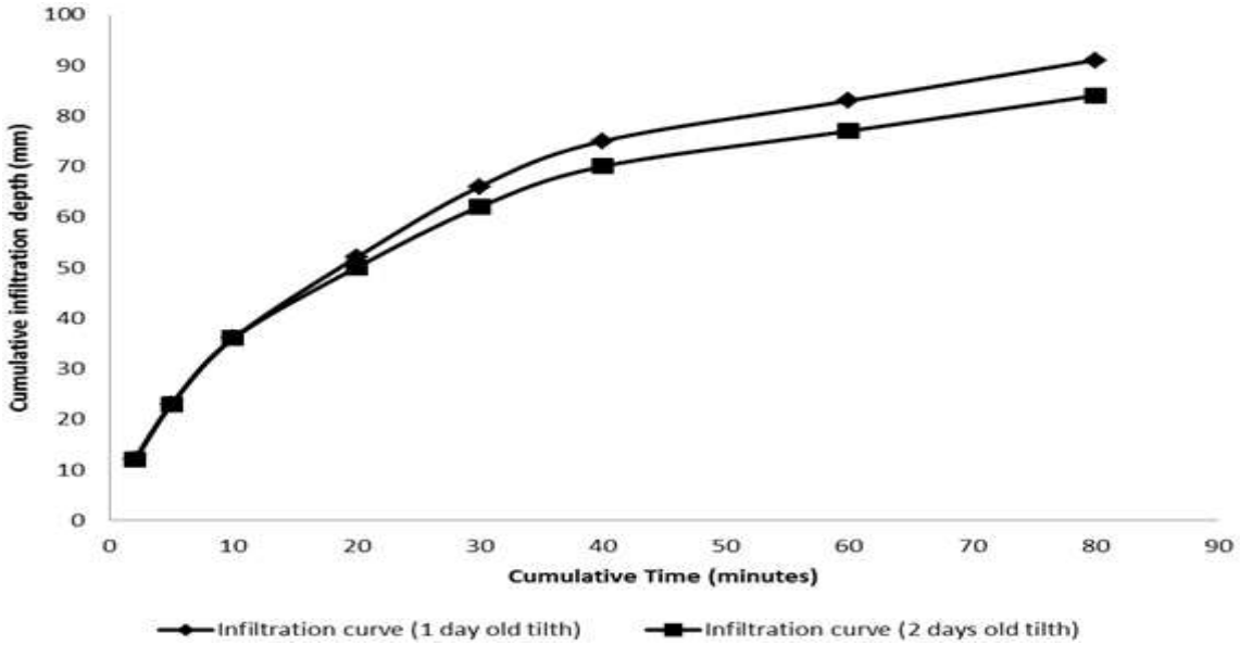
Figure-3. Infiltration Curve for Plough + Harrow Tillage
