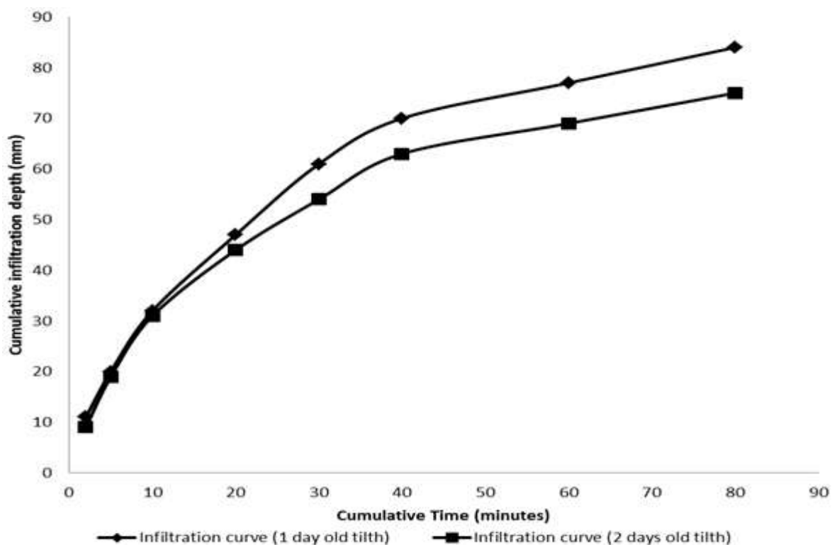
Figure-2. Infiltration Curves for Plough Tillage
